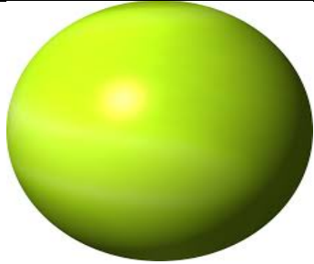
Sphere
