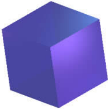
Cube
